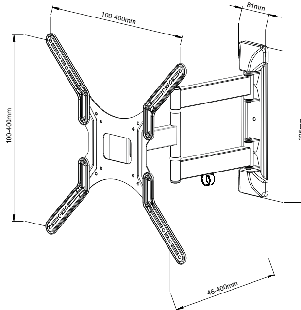
(Schematic Diagram)
